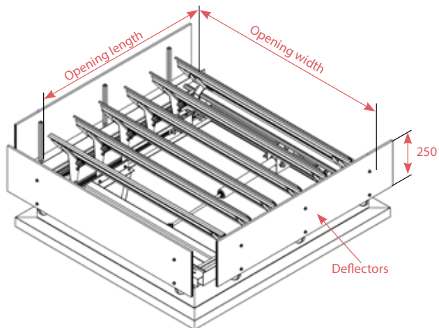
ARCALAM® ÉVOLUPNEU Type: Without Apron with deflectors
