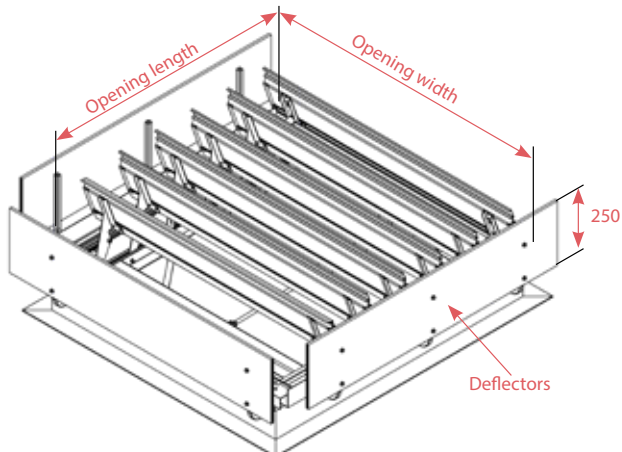
ARCALAM® ÉVOLUPNEU Type: Without Apron with deflectors
