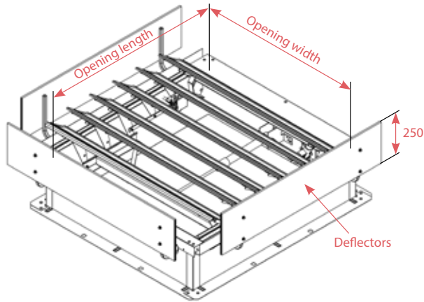
ARCALAM® ÉVOLUPNEU Type: Aluminium Adapter Plate with deflectors
